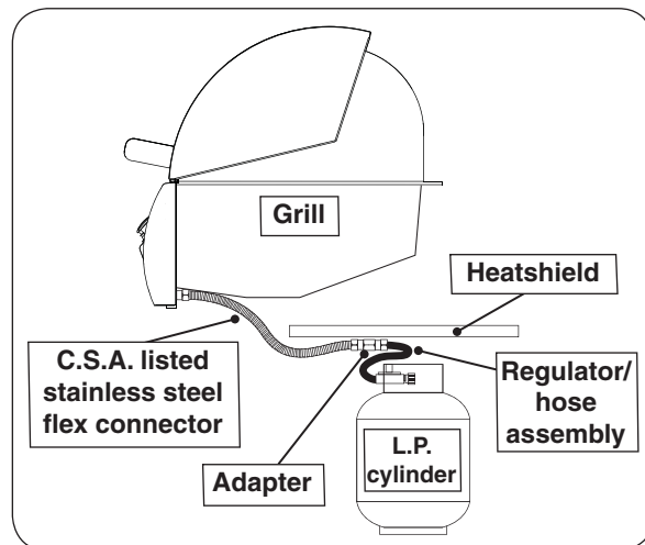
Fig. 13-2 Propane cylinder orientation
