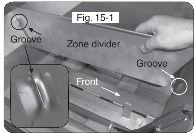
Fig. 15-1 Install zone dividers
