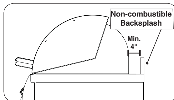
Fig. 11-5 Backsplash clearance
