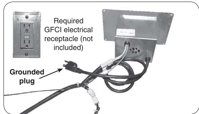
Fig. 16-1 Power supply detail
