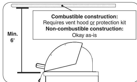
Fig. 11-1 Overhead requirements
