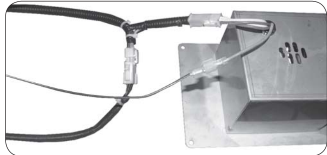
Fig. 16-2 Wire connections
